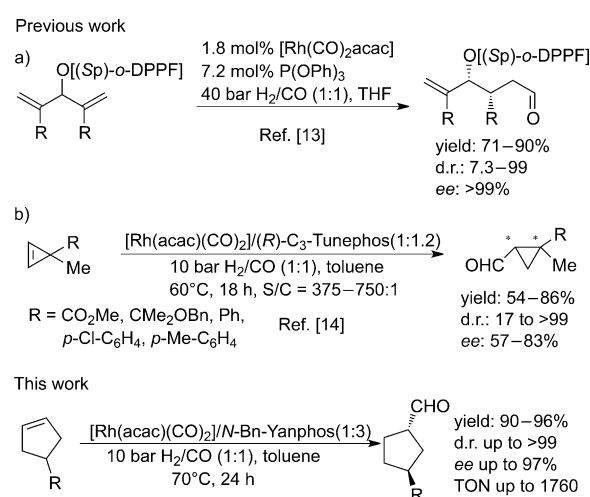
Scheme 1. Examples of desymmetrizing hydroformylation. acac = acetylacetonate, DPPF = 1,1'-bis(diphenylphosphino)ferrocene, THF = tetrahydrofuran, TON = turnover number.
